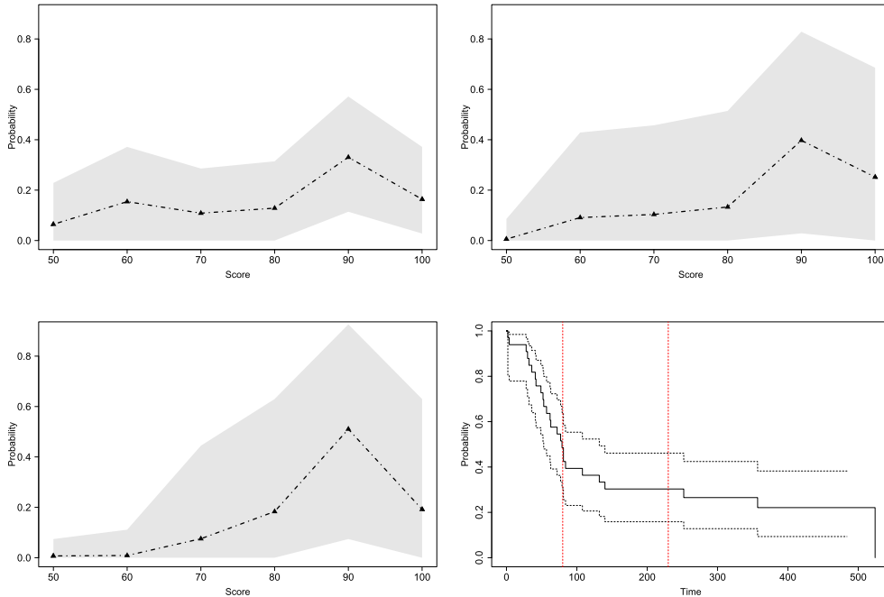
Figure 8: From top left: pmf prediction at 70, 230 and 550 days after the experiment. Bottom right: Kaplan-Meier estimate of the survival times up to time 550.
