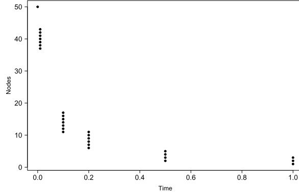
Figure 4: Nodes in \{0, \dots, 50\} (black dots) with probability of being reached by the death process bigger than .05 after lags .01, .1, .2, .5 and 1 (horizontal axis). Starting with mass 1 at the point 50, only a handful of nodes have significant mass after these lags.
