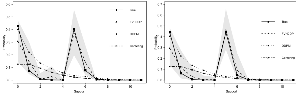
Figure 7: One- (left) and two-step-ahead prediction (right) based on 5 data collection times, with 95% pointwise credible intervals.
