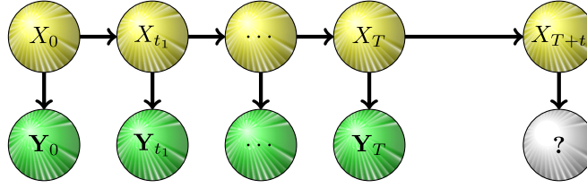
Figure 2: The predictive problem depicted as a graphical model. The upper yellow nodes are nonobserved states of the infinite-dimensional signal, the lower green nodes are conditionally independent observed data whose distribution is determined by the signal, the light gray node is the object of interest.
