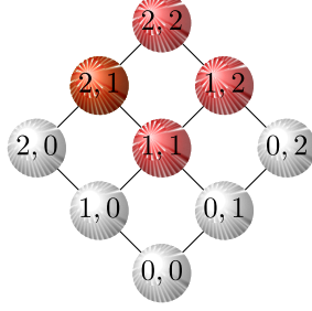
Figure 1: Red indices in the graph identify active mixture components at time T , i.e. the set \mathbf{M} in (2.5), corresponding to points \mathbf{m} \in \mathbb{Z}_+^K with positive weight. In this example K = 2 , and the graph refers to \mathbf{M} at time T = 1 if we observe \mathbf{Y}_0 = (y_1^*, y_2^*) = \mathbf{Y}_1 .
