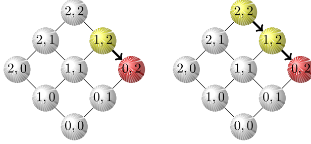
Figure 3: The weight associated to an index \mathbf{n} \in L(\mathbf{M}) at time T + t is determined by the probability that the death process reaches \mathbf{n} from any active index \mathbf{m} \in \mathbf{M} at time T . For \mathbf{M} as in Figure 1, the weight of the mixture component with index \mathbf{n} = (0, 2) , i.e., no atoms y_1^* and 2 atoms y_2^* , is the sum of the probabilities of reaching node (0, 2) via the path starting from (1, 2) (left) and from (2, 2) (right).
