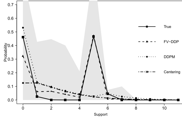
Figure 6: One-step-ahead prediction and 95% pointwise credible intervals, based on 15 data collection times.
