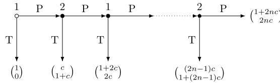
Fig. 3. Game 3: Centipede.
