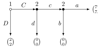
Fig. 1. Game 1: A CI game with sequential moves by player 2.
